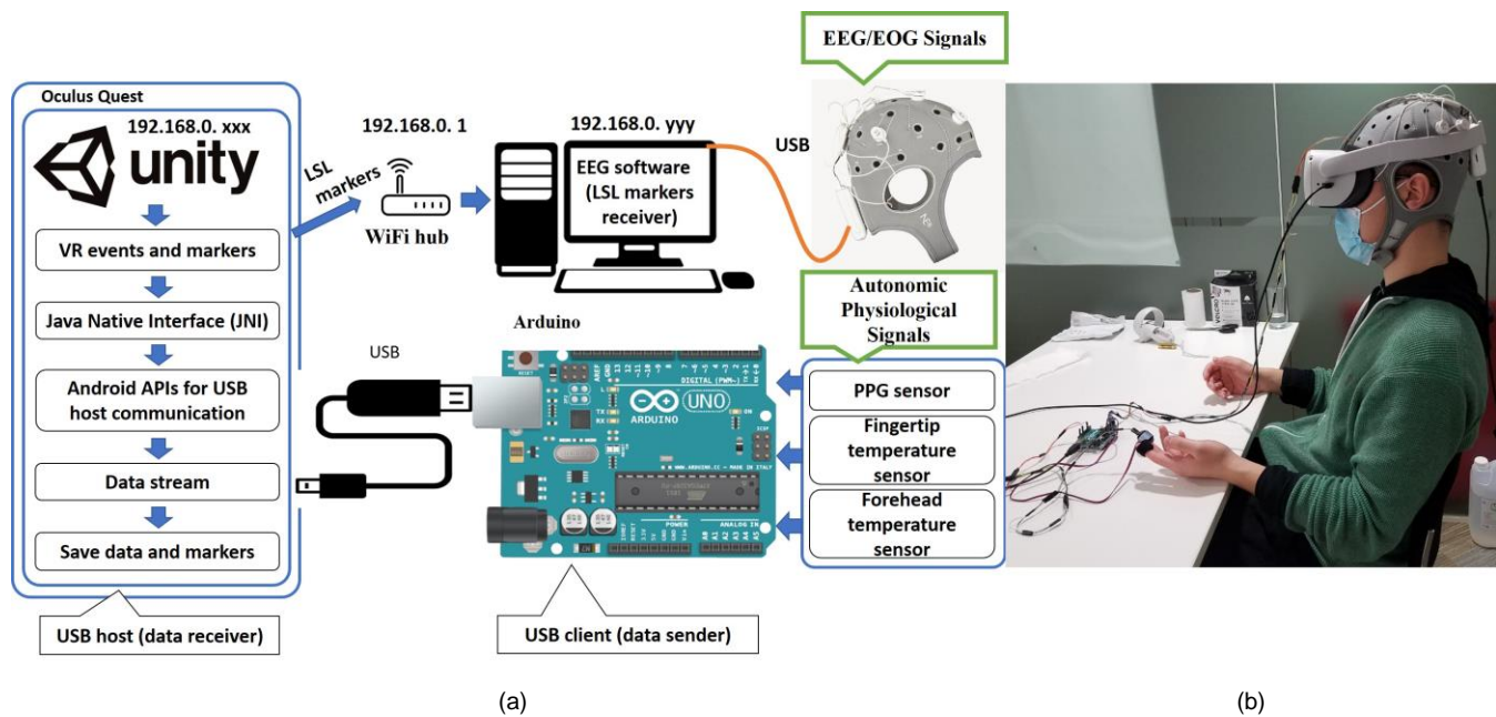
Fig. 1. (a) Block diagram of the proposed multimodal sensing system, where the Lab streaming layer (LSL) protocol was used to synchronize VR events with EEG data collection software. The LSL protocol, developed by University of California, San Diego a decade ago, can ensure sub-millisecond accuracy as long as both the LSL host (marker sender) and client (receiver) are in the same local network. The LSL's applicability in combined VR-EEG settings has been confirmed in our previous studies [25], [40]. For the physiological sensing platform, USB communication between Arduino and Oculus Quest was developed using middleware Java Native Interface (JNI) bindings. JNI was used to enable Java code to be called by a non-Java platform so that our VR application can access the hardware layer of Quest and stream all physiological data from Arduino's USB interface into Quest and attach event markers to these data and directly store them as CSV files inside Quest. "Attaching event markers" was executed by two lines of consecutive C# code immediately after the task session started or after every 1-min FMS score reported. The latency was in the order of tens of milliseconds, so there were no meaningful system delays. (b) Sample experimental environment.
